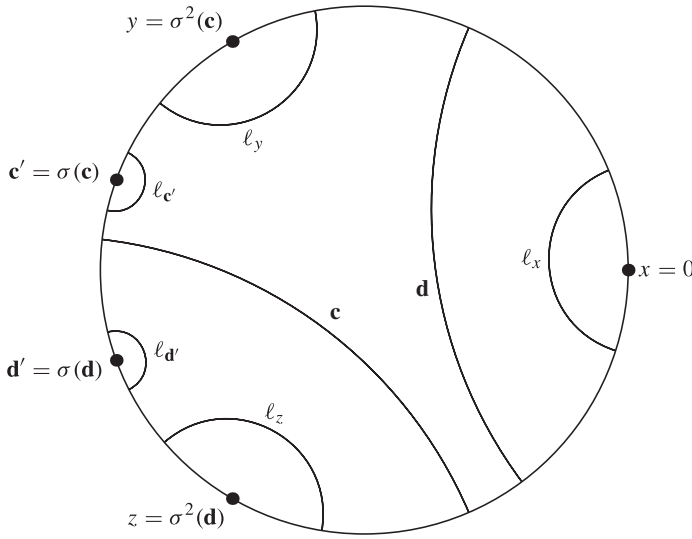
FIGURE 4. A \mathbf{c} -lamination constructed as in the proof of Lemma 3.2.2, with M = 1 and N = 2 .
