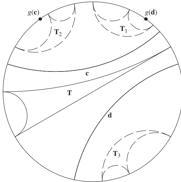
FIGURE 1. Consider the finite dynamical lamination \mathcal{L} = \{\mathbf{c}, \mathbf{d}, \mathbf{T}, g(\mathbf{c}), g(\mathbf{d})\} pictured here and a few possible backward continuations of (\mathcal{L}, g) whose new elements are pictured in dashed lines. It is evident that all backward continuations of (\mathcal{L}, g) adding only a first preimage of \mathbf{T} under \mathbf{d} (like \mathbf{T}_3 , as illustrated) are order isomorphic. However, the choice of a first preimage of \mathbf{T} in the component of \mathbb{S}^1 \setminus \mathbf{c} , containing the last classes g(\mathbf{c}) and g(\mathbf{d}) , is ambiguous; \mathbf{T}_1 and \mathbf{T}_2 illustrate choices giving rise to backward continuations which are not order isomorphic.
