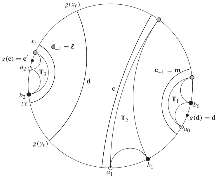
FIGURE 3. A simple \mathbf{c} -lamination. Like-shaded vertices are in the same orbit. The monotone sequence of intervals is ([a_0, b_0], [a_1, b_1], [a_2, b_2], [g(x_\ell), g(y_\ell)]) , g^2(\mathbf{m}) = \mathbf{c}' , and r = 2 . The monotone itinerary is (C, C, D, D) , where C denotes the \{\mathbf{c}, \mathbf{d}\} -unlinked class whose boundary is \mathbf{c} , and likewise D for \mathbf{d} .
