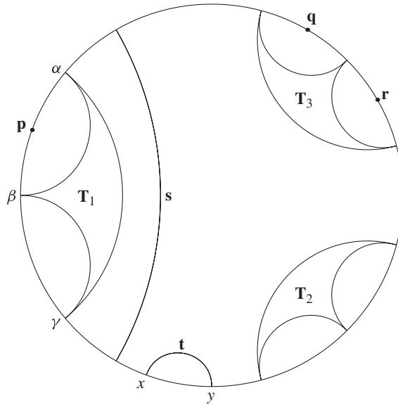
FIGURE 2. An illustration of concepts from Definition 2.3.1. The finite lamination in question is \mathcal{L} = \{p, q, r, s, t, T_1, T_2, T_3\} . The triple T_1 is leaf-like, and is adjacent to both the bud p and the leaf s . Its long edge is therefore \{\alpha, \gamma\} , its short edge is \{\alpha, \beta\} , and its empty edge is \{\beta, \gamma\} . The class T_3 is adjacent to both q and r . The triple T_2 is not leaf-like, and is not adjacent to any other class. The arc under the leaf t is [x, y] . There are no arcs under s . The arcs under the different edges of T_1 are [\alpha, \beta] , [\beta, \gamma] , and [\gamma, \alpha] .
