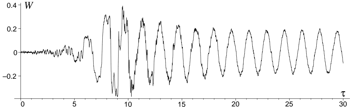
Figure 2: The piston velocity W as a function of time \tau . The same run as in Fig. 1.
