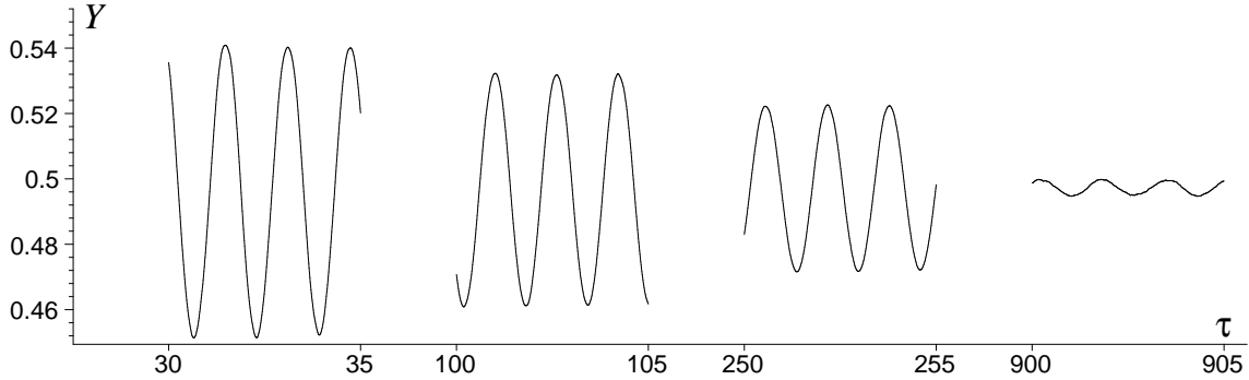
Figure 3: The piston coordinate Y during the intervals (30, 35) , (100, 105) , (250, 255) , and (900, 905) . The same run as in Fig. 1 and 2.
