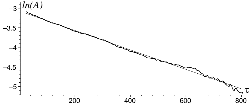
Figure 4: The amplitude A(\tau) on the logarithmic scale: experimental curve (bold) and a linear fit (thin). The same run as the one shown in Fig. 1, 2 and 3.
