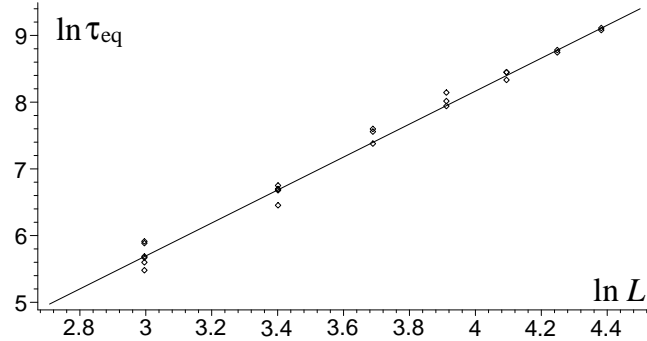
Figure 8: The value \ln \tau_{\text{eq}} as a function of \ln L : experimental points and a linear fit.
