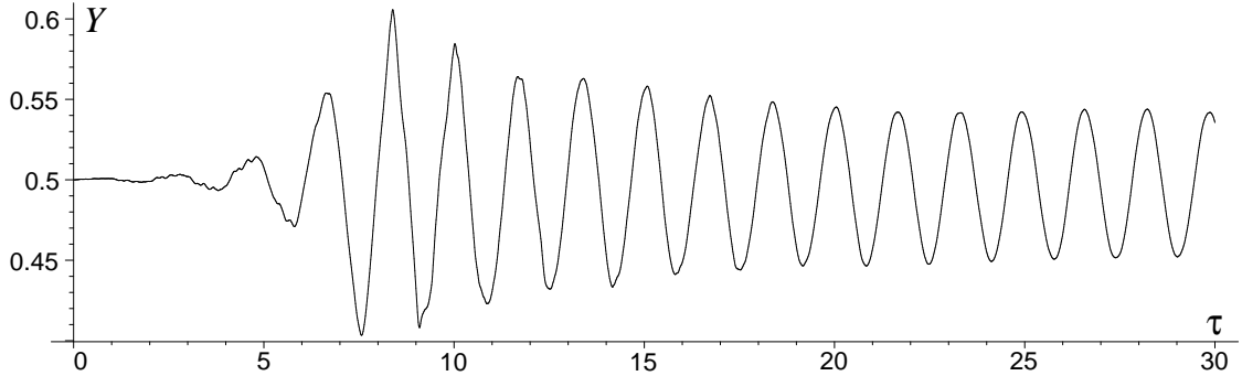
Figure 1: The piston coordinate Y as a function of time \tau . Here L = 100 , N_- = 500341 , N_+ = 499888 .
