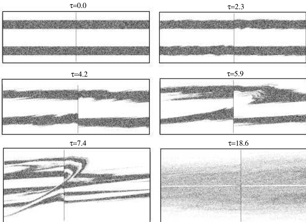
Figure 6: Six snapshots of the empirical gas density (in the x, v plane) at times \tau = 0, 2.3, 4.2, 5.9, 7.4 and 18.6 .
