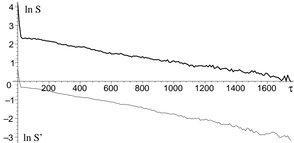
Figure 9: \ln S (thick line) and \ln S' (thin line) as functions of \tau .
