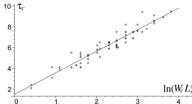
Figure 7: The value \tau_c as a function of \ln(W_c L) : experimental points and a linear fit.
