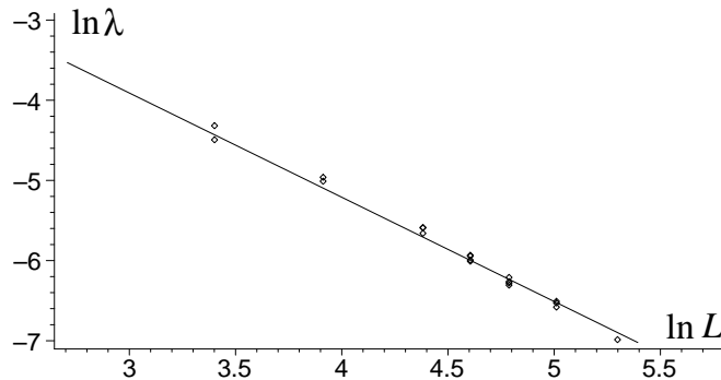
Figure 5: The value \ln \lambda as a function of \ln L : experimental points and a linear fit.
