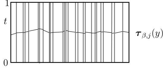
Figure 2: The partition of a rectangle over an H-component W_{\beta,s_0,j} : the irregular line in the middle is the graph of the function \tau_{\beta,j}(y) ; it separates the ‘upper subrectangle’ (of the second type) from lower trapezoids (of the third type).
