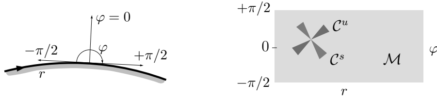
Figure 1: Orientation of r and \varphi and the collision space.
