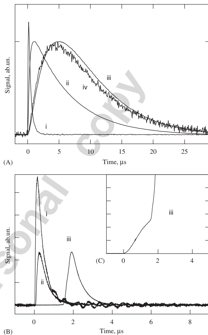
Fig. 5. (A) Kinetics of \text{Cr}:\text{ZnSe} single crystal mid-IR photo-luminescence at \sim 2500 nm under (ii) 1560 nm, (iii) 532 nm, (iv) 355 nm pumping with pump temporal profile shown in (i). (B) Dynamics of \text{Cr}:\text{ZnSe} laser oscillation build-up. Pulse (i) shows the pump pulse. Pulse (ii) shows the temporal profile of the lasing pulse from 1560 nm excitation. Pulse (iii) shows the temporal profile of the lasing pulse from 532 nm excitation. The inset (C) is a blow-up of the build-up part of the temporal profile of the 2500 nm lasing pulse under 532 nm excitation. This plot shows that \sim 2 \mu\text{s} build up time is required before mid-IR lasing occurs under 532 nm excitation.
